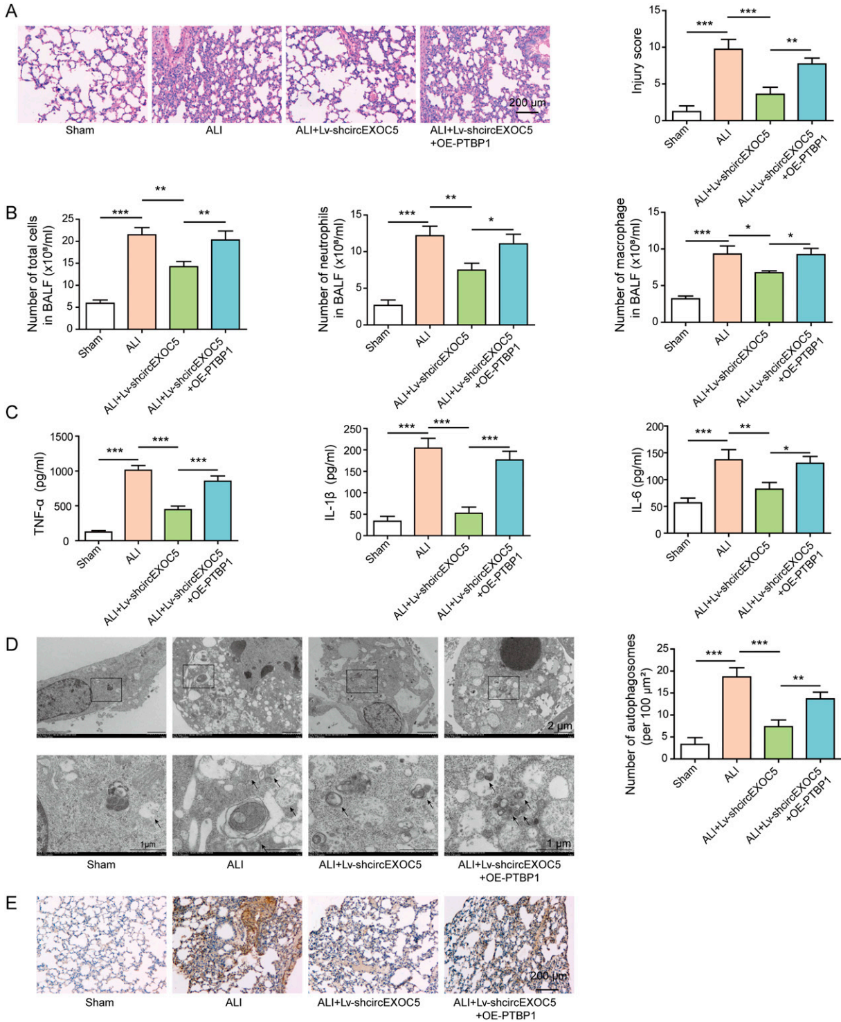
Figure 7. Overexpressing PTBP1 abolished the in vivo preventive benefits of silencing circEXOC5 on acute lung injury. Mice were injected with Lv-shcircEXOC5 or Lv-shcircEXOC5 + OE-PTBP1 before the CLP procedure. (A) Histology of lung tissues from indicated groups was examined by HE staining and scored for lung injury. Scale bar: 200 μm. (B) Numbers of total cells, neutrophils, and macrophages in BALF were quantified. (C) Production of TNF-α, IL-6, and IL-1β in BALF was measured by ELISA. (D) Autophagosomes in lung tissues were observed under a transmission electron microscope, with the number counted from indicated groups. Scale bar: 2 or 1 μm. (E) Runx2 expression was detected by immunohistochemical analysis in indicated lung tissues. Scale bar: 200 μm. * P < 0.05, ** P < 0.01, and *** P < 0.001.
