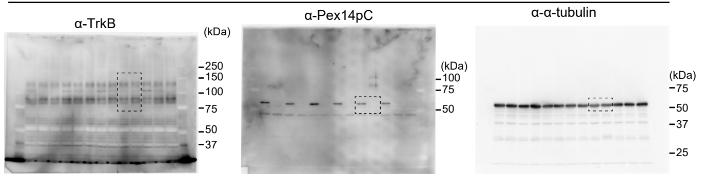
Full unedited gel for Figure 6 E
