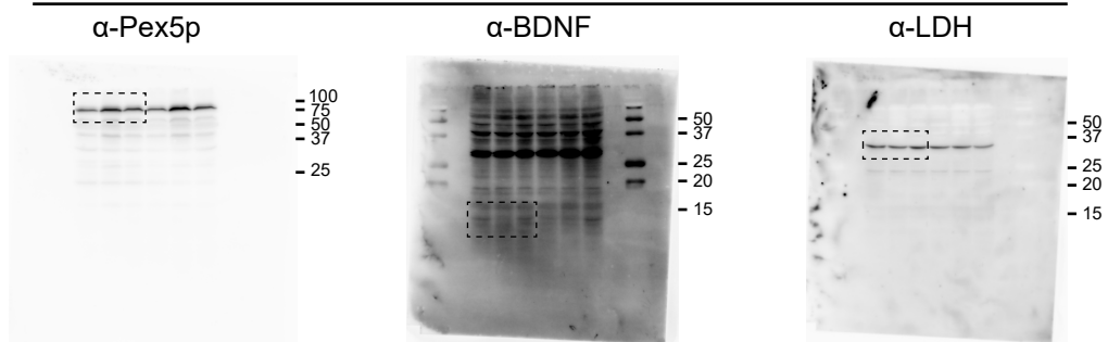
Full unedited gels for Figure 4 E
