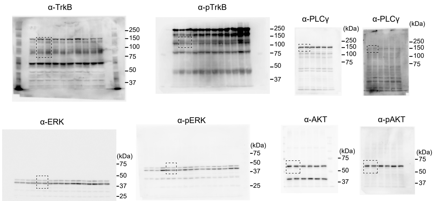
Full unedited gel for Figure 7 A
