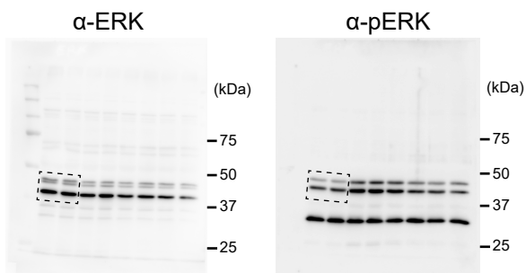
Full unedited gel for Figure S4 D
