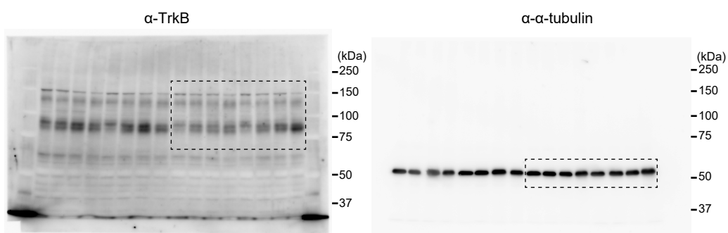
Full unedited gel for Figure S3 F
