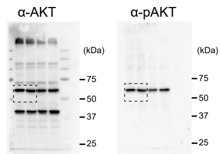
Full unedited gel for Figure S4 E
