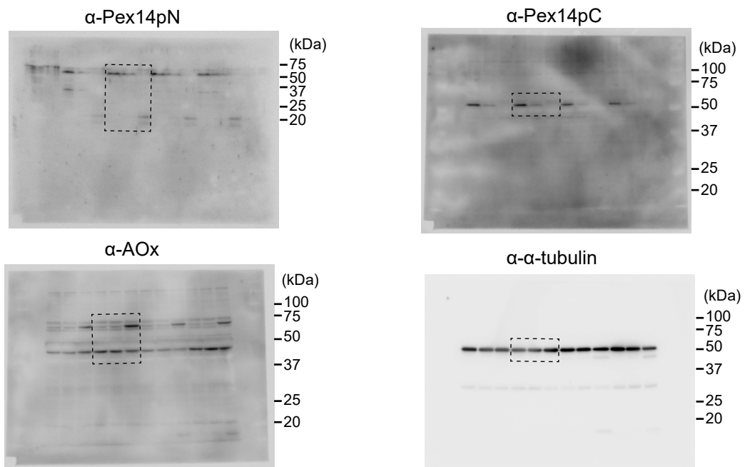
Full unedited gel for Figure 2 E
