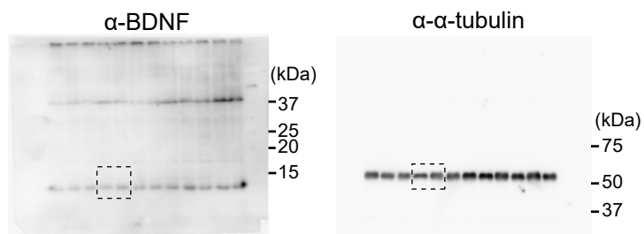
Full unedited gel for Figure 8 H
