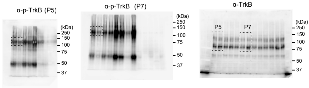
Full unedited gel for Figure S3 H
