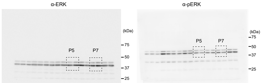
Full unedited gel for Figure S3 I
