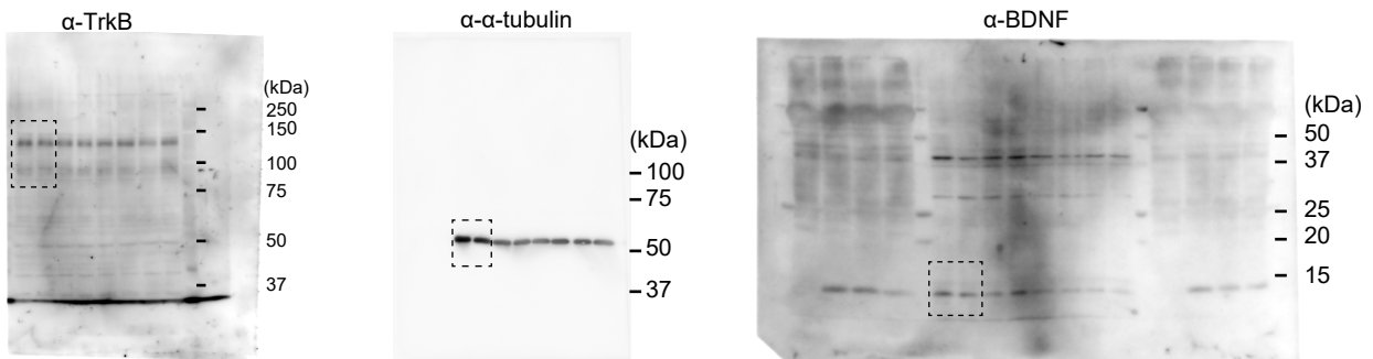
Full unedited gel for Figure S4 A
