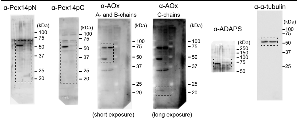
Full unedited gel for Figure S3 F
